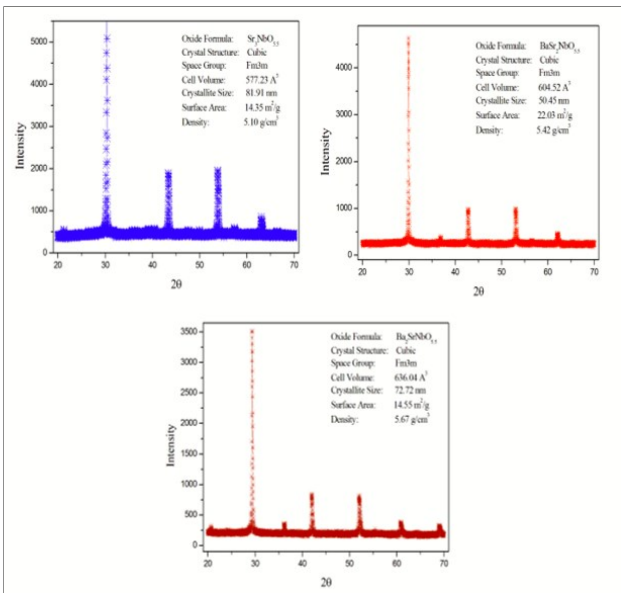
Figure 1 the XRD patterns of \text{Sr}_3\text{NbO}_{5.5} , \text{BaSr}_2\text{NbO}_{5.5} and \text{Ba}_2\text{SrNbO}_{5.5} .
