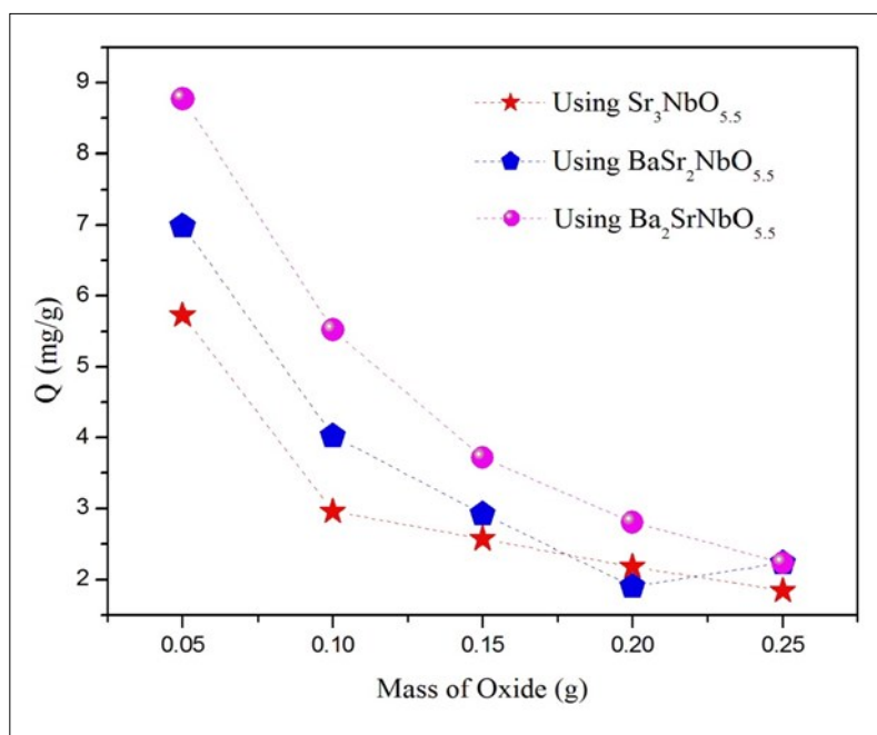
Figure 4. The effect of adsorbent mass on the removal. The time, volume, concentration and pH of dye solutions are 150min, 50ml, 10ppm and 5.1 respectively.
