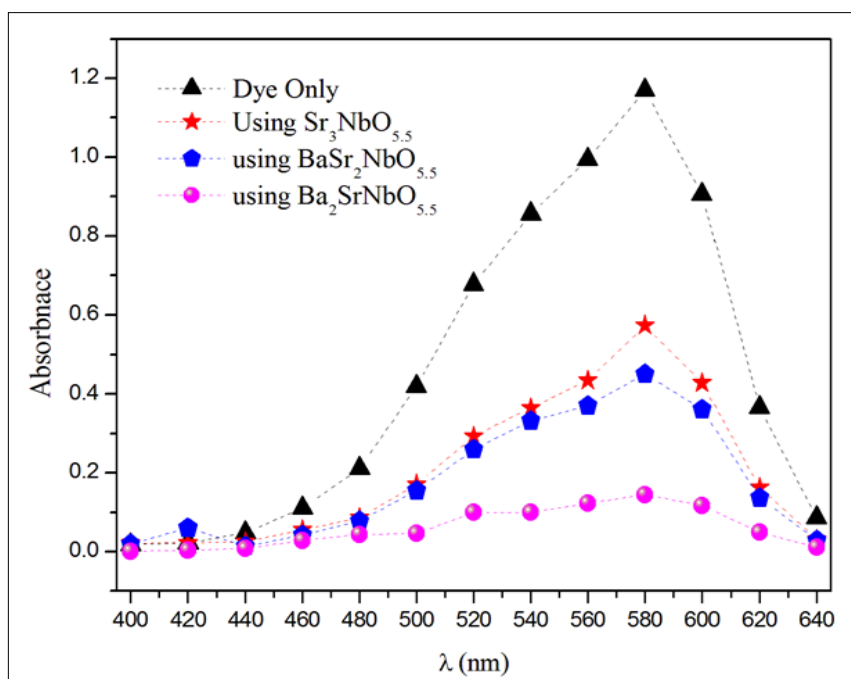
Figure 3. The wavelength dependence of absorbance for MV solution. The time, volume, concentration, adsorbent mass and pH of MV solution are 150 min, 50ml, 10ppm, 0.1 g and 5.1 respectively.
