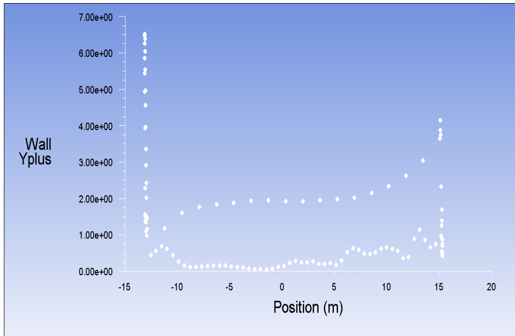
Figure 1. Plot for determining the Y+ on the blade profile.
