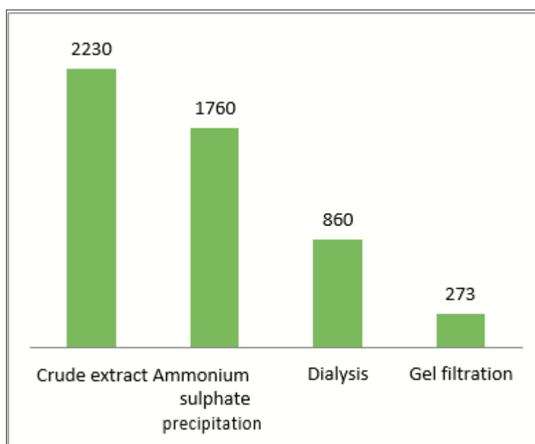
Figure7. Enzyme Activity ( From Crude Enzyme To Partial Purification)
